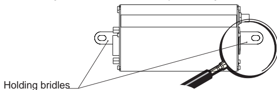
Figure 2 Modem mounting
